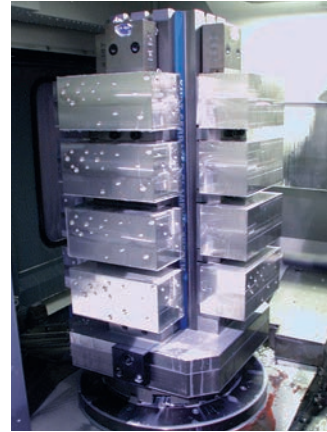
SeraLock Towers for high density
