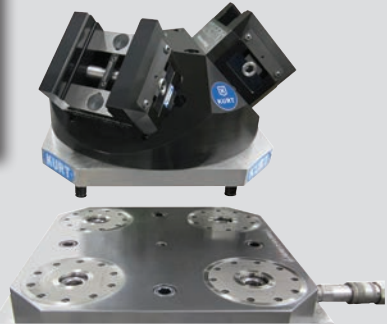
5 axis vises on Pyramid platform using zero-point system.
