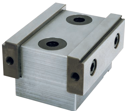
Stationary Jaw MLS351
